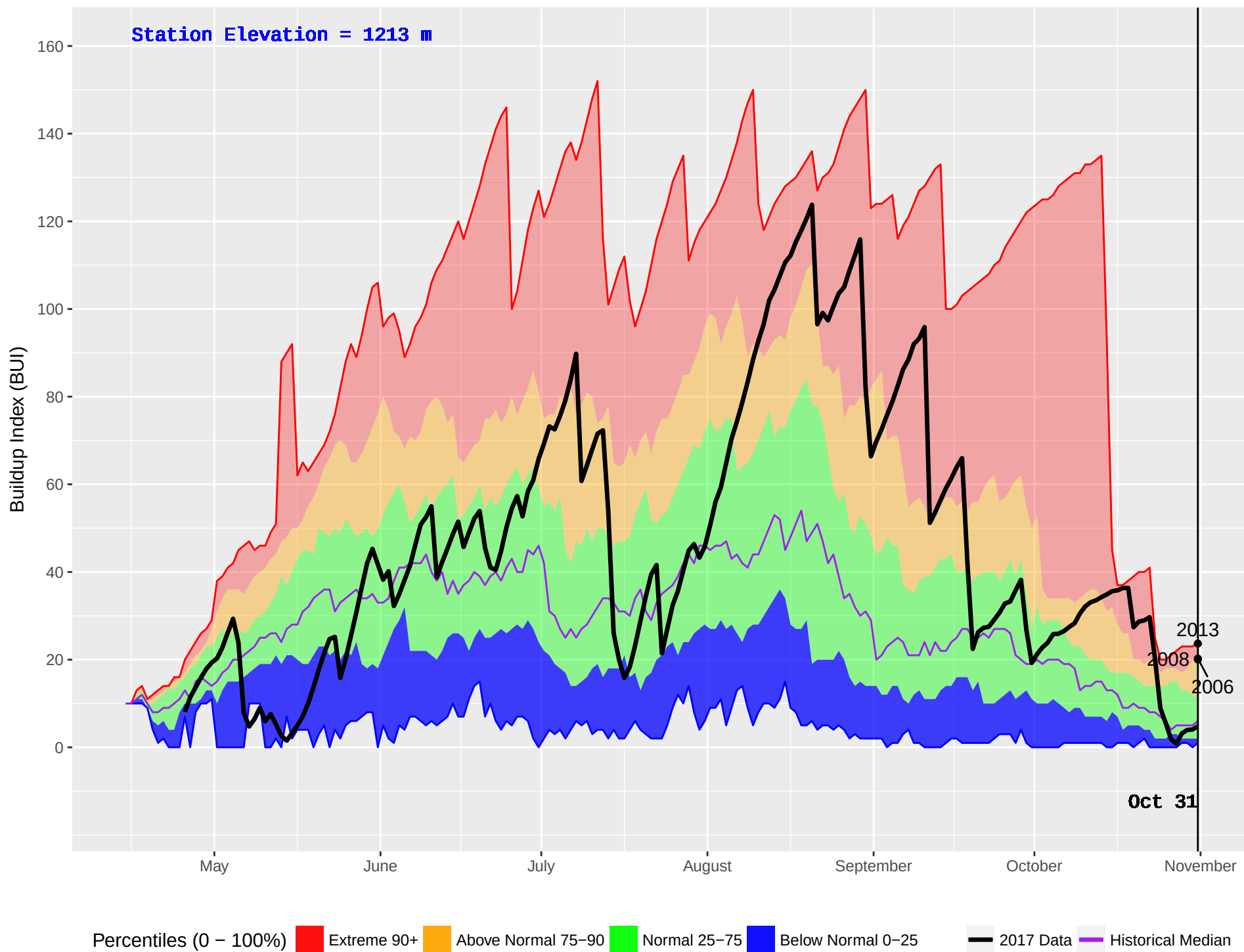
INGENIKA POINT (145) : Historical (1971–2016) and Current (2017) Noon Buildup Index (BUI)
